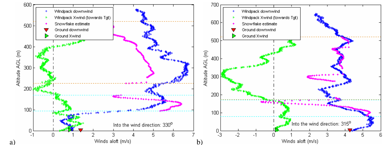
Fig. 24 Windpack 2 data versus Snowflake estimate for Drop #4 (a) and Windpack 3 data versus Snowflake estimate for Drop #6 (b).
